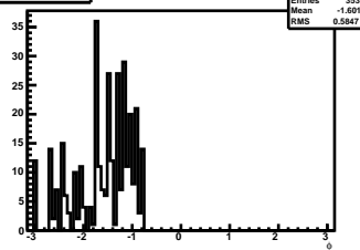
L2Seed Muon \phi
