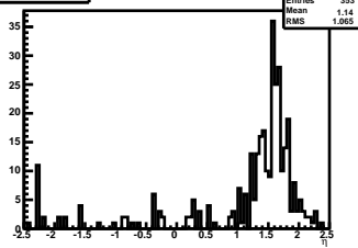
L2Seed Muon \eta
