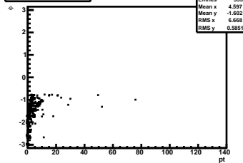
L2Seed Muon pt vs \phi
