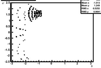
L2Seed Muon \eta vs \phi
