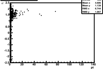
L2Seed Muon pt vs \eta
